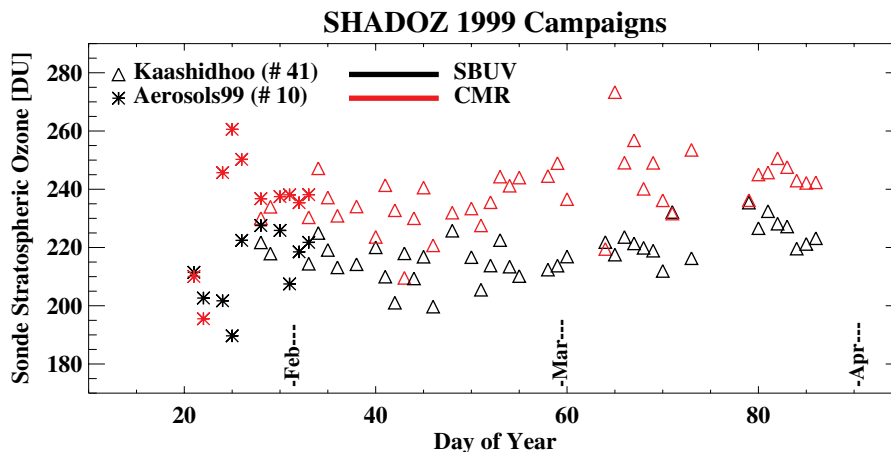
Figure 4. Stratospheric ozone computed from soundings at Kaashidhoo during INDOEX (triangles) and from Aerosols99 cruise (launches to \pm 20^\circ latitude, asterisks). Stratospheric column amount computed by subtracting integrated tropospheric ozone from the sonde total ozone. Campaign data are color-coded in black (SBUV) and red (CMR) to illustrate the two extrapolation techniques.
